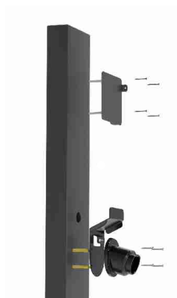
Figure 4-11 Holders Installation
