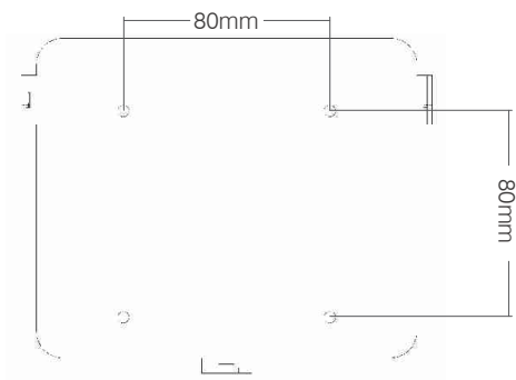
Figure 4-5 Mark Hole Position
