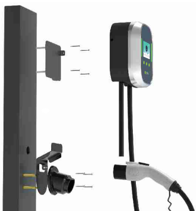
Figure 4-9 General Installation Drawing
